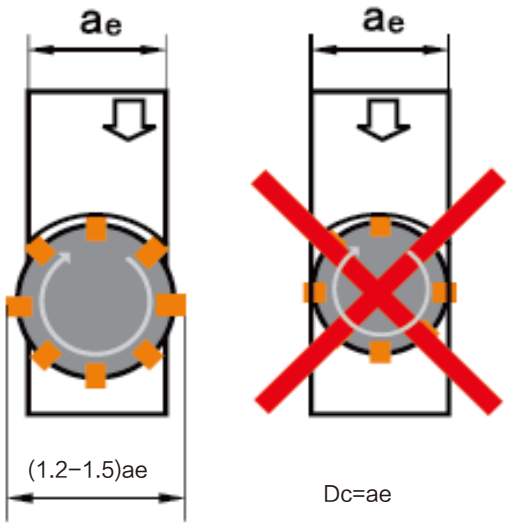
面铣中切宽与刀具切削直径的选择 Selection of Cutting Width and Tool Cutting Diameter in Face Milling
